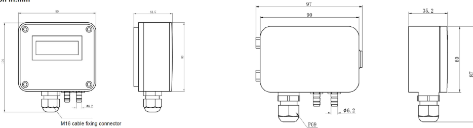
Dimension in:mm
